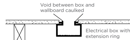
Plan Outlet Box Detail
