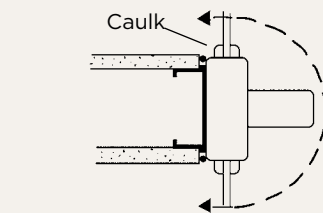
Plan Typical Partition Mullion Intersection
