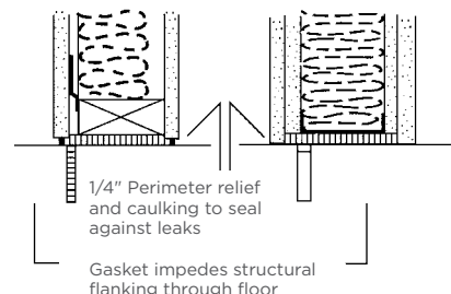
Elevation Typical Floor-Ceiling or Roof Detail
