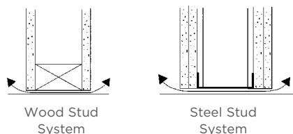
Elevation Under and Over Partitions
