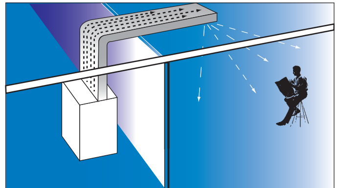
Figure 20: Significant noise reduction can be obtained by lining sheet metal ducts with fiberglass duct liner, or by fabricating duct systems of fiberglass duct board.
