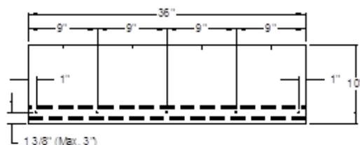
FIGURE 1—SHINGLE PROFILES AND FASTENER PATTERNS (Continued)
