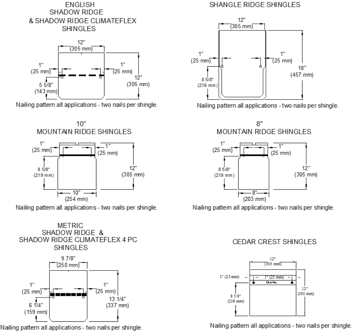
FIGURE 1—SHINGLE PROFILES AND FASTENER PATTERNS (Continued)
