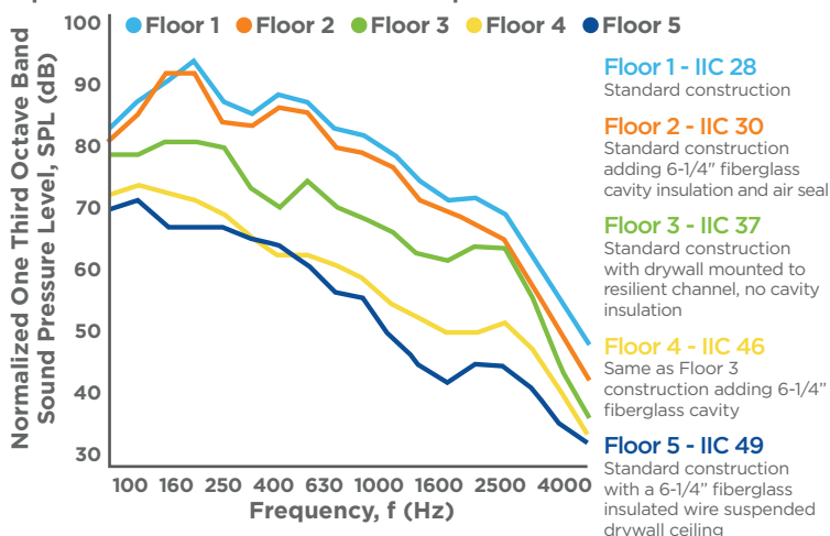
Impact Sound Transmission Data Comparison of Wood Joist Floors
