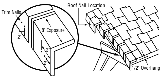
Figure 11-18: Rake edge application
