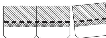
Figure 11-12: Shadow Ridge accessory shingles detach easily from three-piece units to make 72 individual cap pieces.
