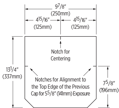
Figure 11-15 : Each Shadow Ridge® shingle has a centering notch and two side-alignment notches to help ensure proper placement
