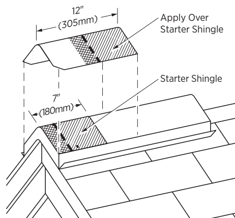
Figure 11-13: Apply a full cap shingle over the starter piece, flush with the bottom and side edges of the starter.
