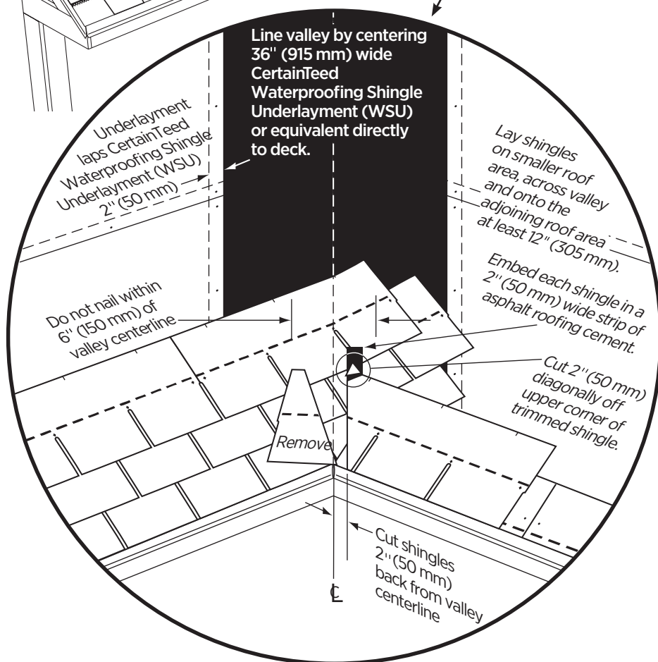
Figure 11-9: Highlight of closed-cut valley details.
