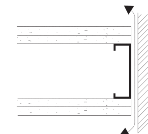
Plan Metal Stud Around Flanking Partition Ends
