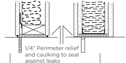
Elevation Typical Floor-Ceiling or Roof Detail
