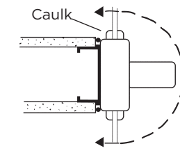
Plan Typical Partition Mullion Intersection
