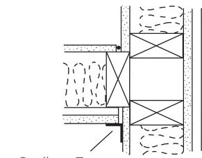
Plan Intersection With Exterior Wall
