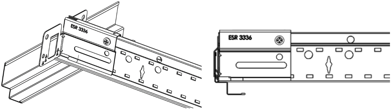
FIGURE 7A – SEISMIC PERIMETER CLIP FIXED WALL SETUP FOR SEISMIC DESIGN CATEGORIES D, E, AND F IN SECTION 4.2.1 (SHADOW MOLDING SM1000)
