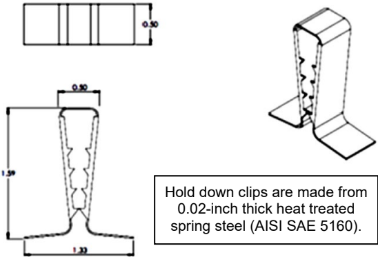
FIGURE 20—HOLD DOWN CLIPS FOR SLOPED CEILINGS
