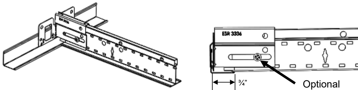
FIGURE 4A – SEISMIC PERIMETER CLIP FREE WALL ASSEMBLY IN SECTION 4.2.1
