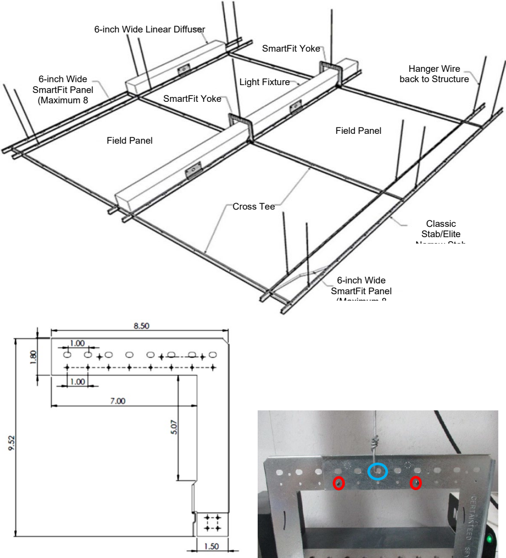
FIGURE 19—SMARTFIT YOKE SYSTEM (SFYK)
