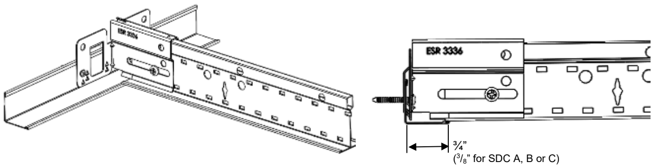
FIGURE 4B – SEISMIC PERIMETER CLIP (CTSPC-2 WITH TWO SCREW ATTACHMENT) FREE WALL ASSEMBLY WITH WALL ANGLE (WA14-14) IN SECTIONS 4.2.2, 4.2.6, 4.2.7, 4.2.8, 4.2.9, 4.2.10, 4.2.11 AND 4.2.12
