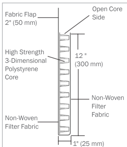
Product Cross-Section
