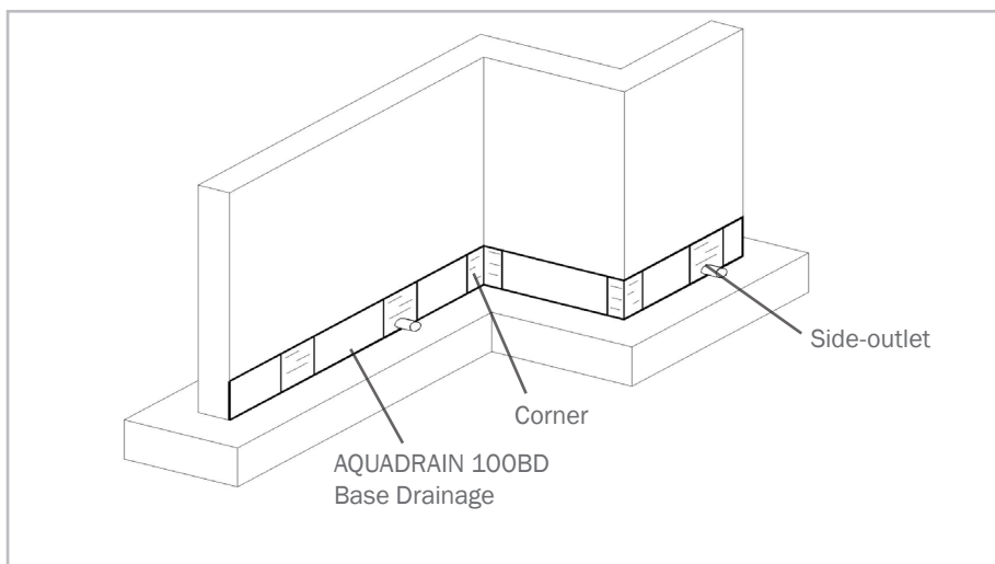
AQUADRAIN 100BD Drainage System Illustration
