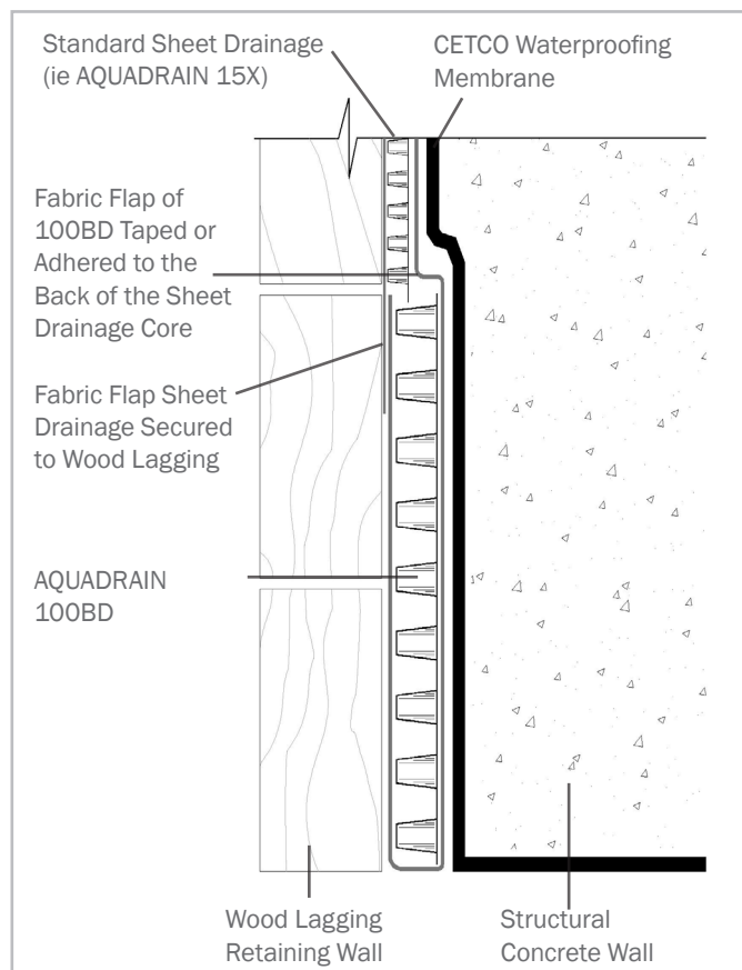
AQUADRAIN 100BD Drainage System Illustration
