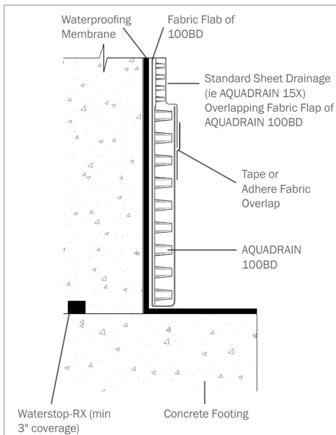
AQUADRAIN 100BD Drainage System Illustration
