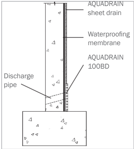
RETAINING WALL
