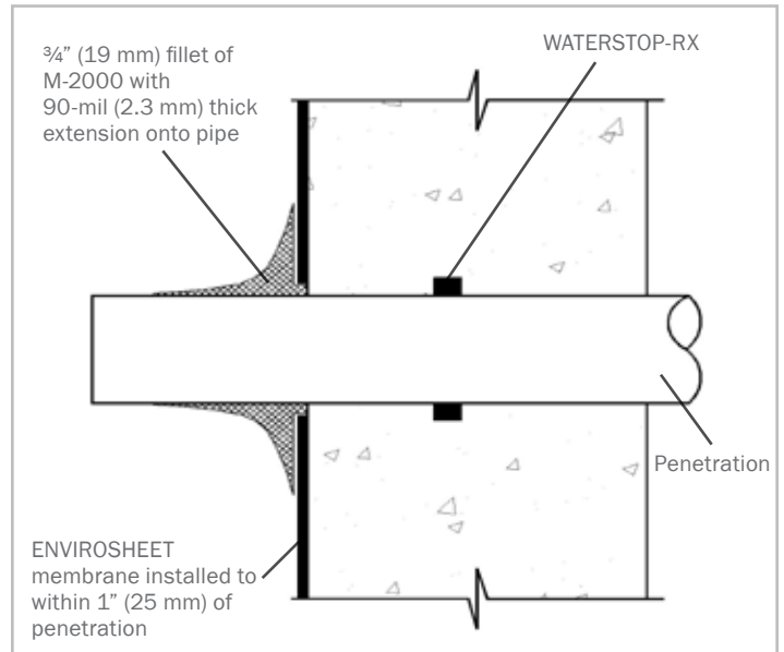
Detail 5 – Single poured-in-place penetration detail
