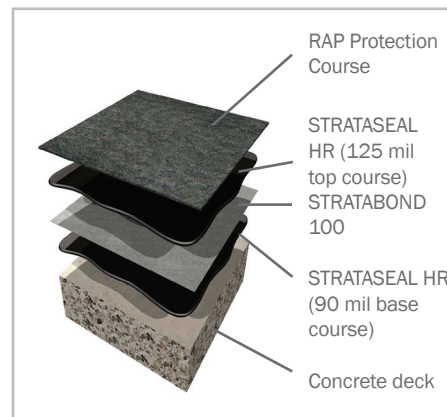
215-mil Thick reinforced membrane
