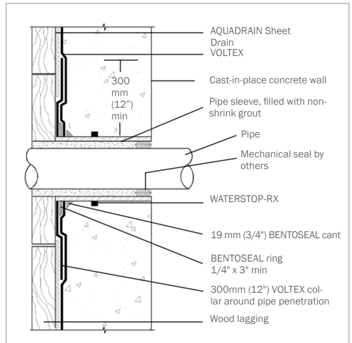
Figure 2.2 - SLEEVED WALL PENETRATION - Cut and secure VOLTEX tightly around penetrations and then apply BENTOSEAL 19 mm (3/4") ring around penetration and extend over membrane a min. 75 mm (3")
