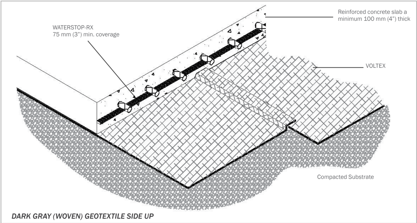
Figure 1.4 - VOLTEX installed directly over compacted earth/gravel substrate requires a minimum 100 mm (4") slab
