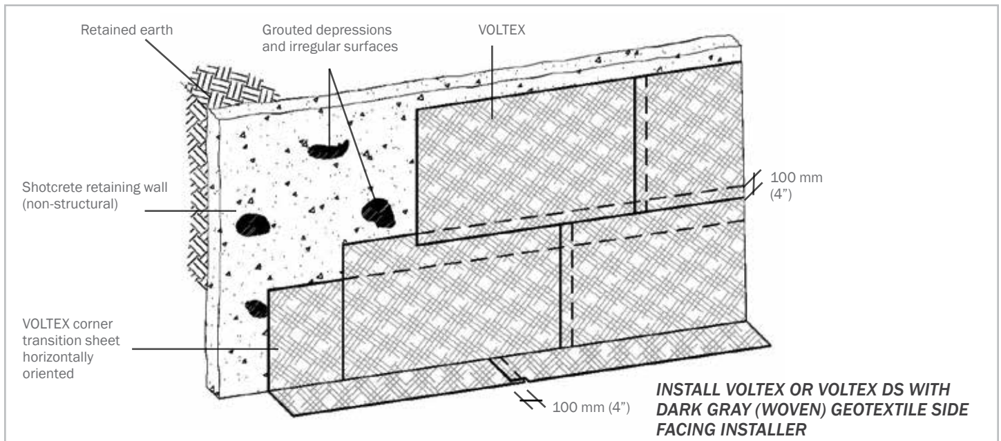
Figure 2.18 – VOLTEX installation over an earth formed shotcrete retaining wall prior to cast-in-place concrete wall
