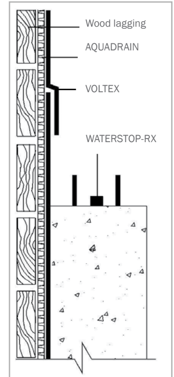
Figure 2.8 – AQUADRAIN used to cover gaps in lagging less than 63 mm (2.5"). (Cast-in-place concrete wall)
