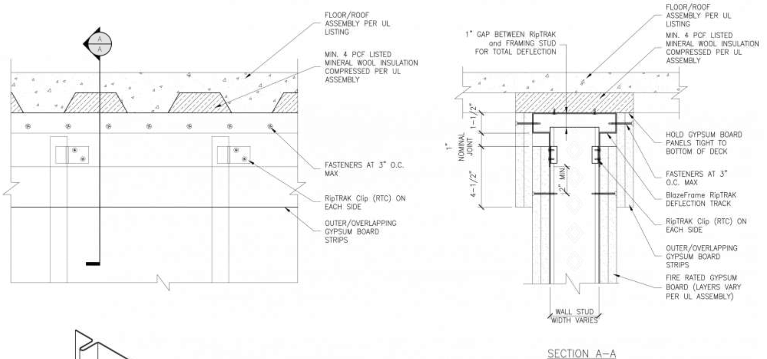
HEAD OF WALL DETAIL RT2-2-UD-2-ALT UL LISTED FLOOR/ROOF ASSEMBLY W/ UNPROTECTED DECK (UD) - MINERAL WOOL FILL
