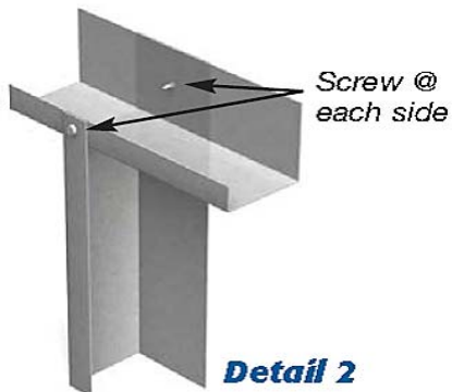
Figure 2 - Construction Detail - Framing
