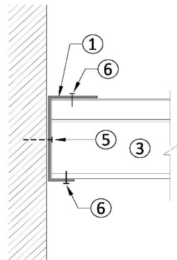
Figure 4 - C-T Stud to J-Runner Connection
