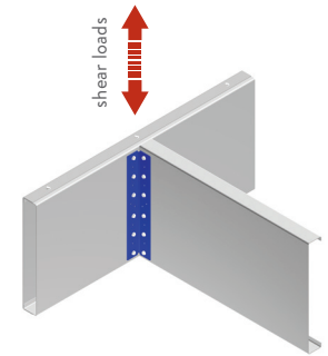
Joist-to-Joist Connections
