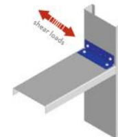
Sill-to-Jamb Connections
