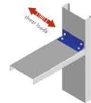
Sill-to-Jamb Connections
