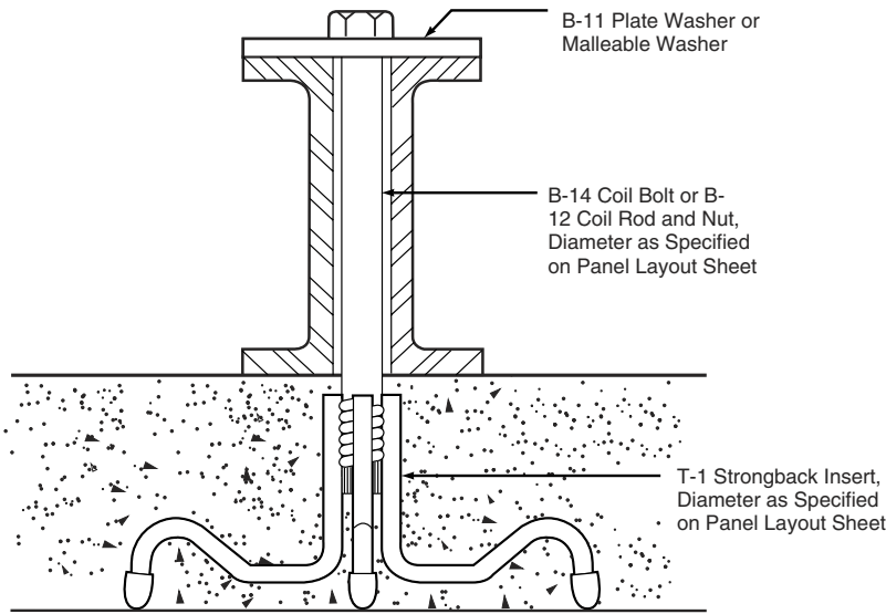
Single Strongback Insert and Bolt
