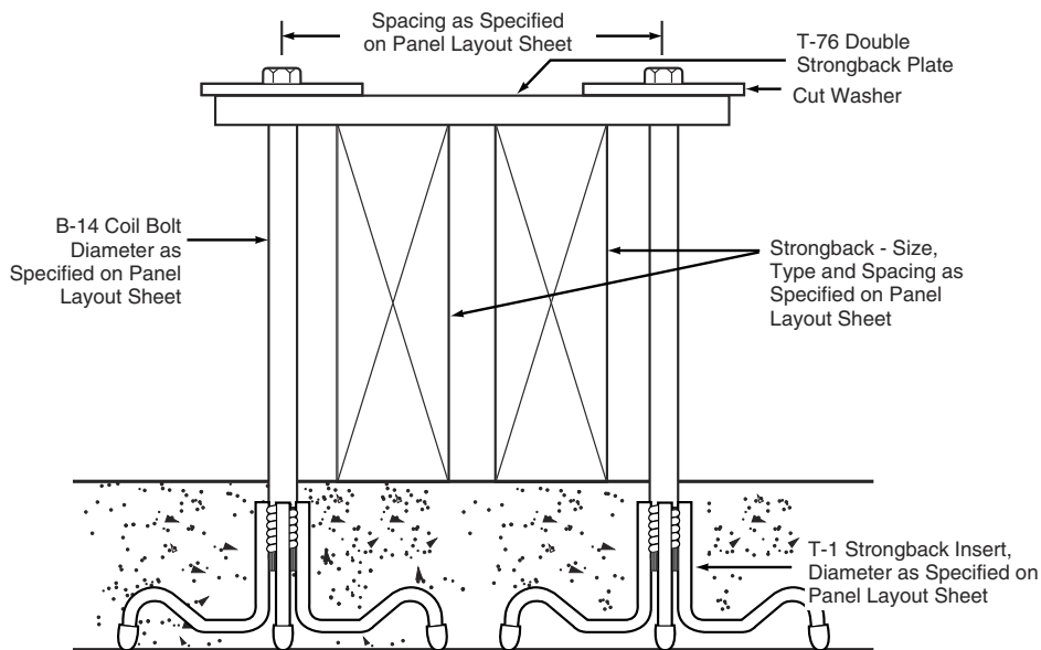
Double Strongback Insert and Bolt
