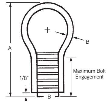
F42 Loop Ferrule Insert
