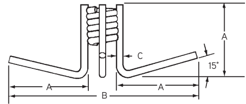
F53 Thin Slab Coil Insert
