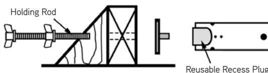
Reusable Recess Plug
