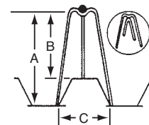
CHC-Continuous High Chairs for Metal Decking
