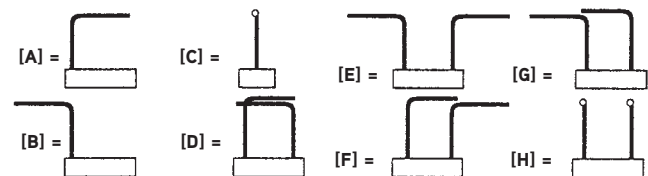
Anchor Direction Legend
