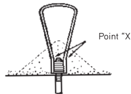
Dotted line indicates line of probable concrete failure Point "X" - point of possible strut fracture.
