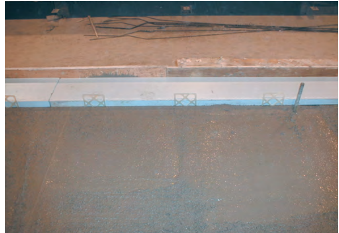
Delta Ties inserted into the first wythe — the exterior wythe — along the edge of the second wythe — the rigid insulation.
