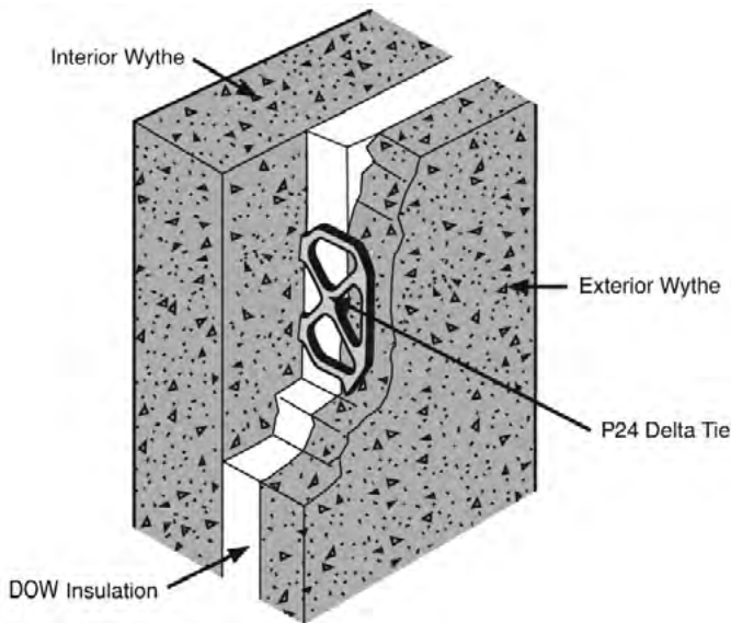
Delta Ties inserted into the first wythe — the exterior wythe — along the edge of the second wythe — the rigid insulation.
