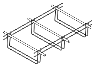
Type "D" Expansion Basket
