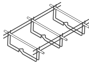
Type "D" Contraction Basket
