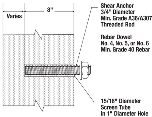
FIGURE 1—CONFIGURATION A (SHEAR ANCHOR OR REBAR DOWEL) 1
