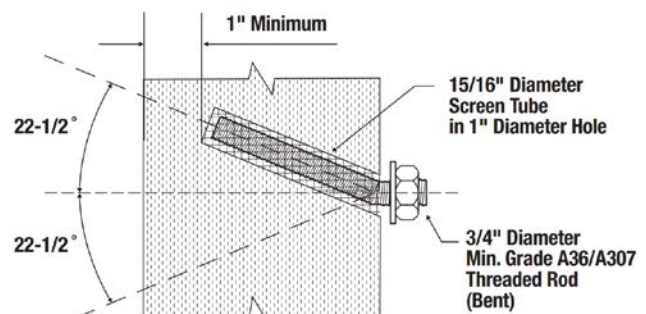
FIGURE 2—CONFIGURATION B (22½-DEGREE COMBINATION ANCHOR) 1
