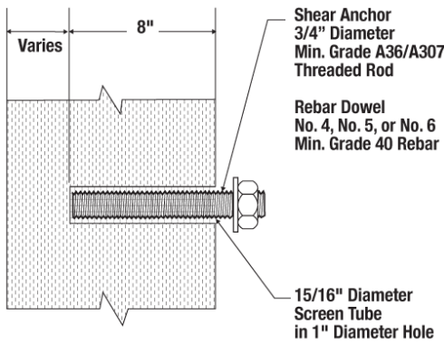
FIGURE 1—CONFIGURATION A (SHEAR ANCHOR OR REBAR DOWEL) 1
