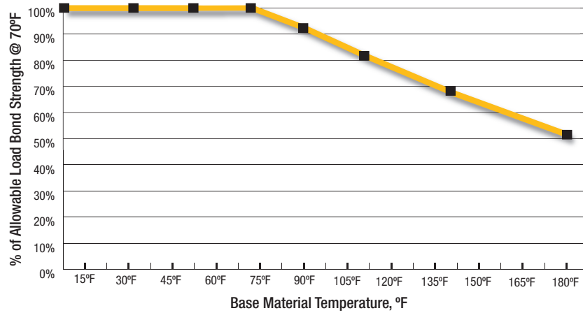
In-Service Temperature Chart For Allowable Load Capacities (based on bond strength/concrete capacity)
