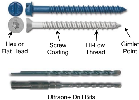
FIGURE 2—ULTRACON+ SCREW ANCHORS AND DRILL BITS
