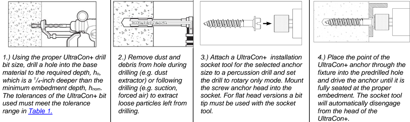
FIGURE 3—ULTRACON+ INSTALLATION INSTRUCTIONS
