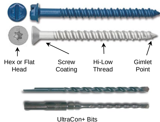
FIGURE 2—ULTRACON+ SCREW ANCHOR AND DRILL BITS
