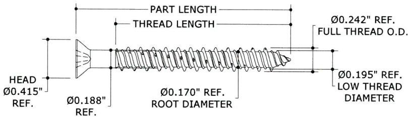
3 4 NTS SIDE VIEW 1/4" TRIMFIT FLAT HEAD (TFH)
