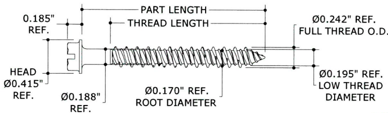
4 4 NTS SIDE VIEW 1/4" HEX WASHER HEAD (HWH)
