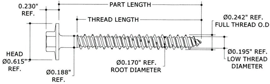
1 4 NTS SIDE VIEW 1/4" HEX FLANGE HEAD (HFH)
