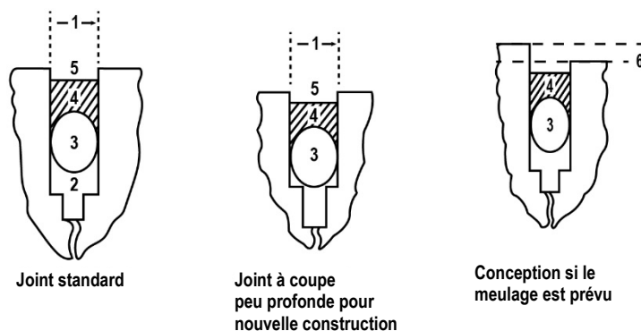
Figure 1: Bonne conception du joint
