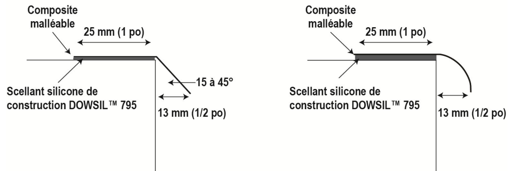
Figure 1: Conception de larmiers
