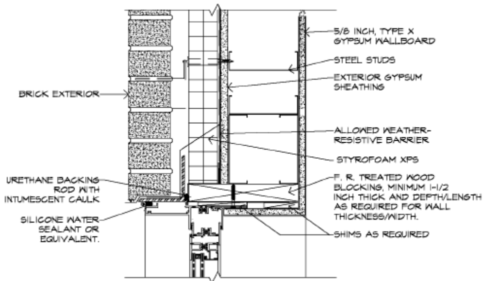
FIGURE 7—WINDOW HEAD DETAIL—FRTW WOOD BLOCKING—FRAMED WALL
