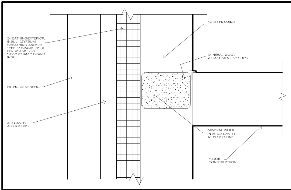
FIGURE 4—FLOORLINE FIRESTOPPING
