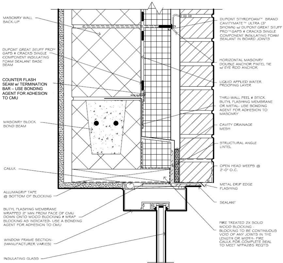
FIGURE 6—WINDOW HEAD DETAIL—FRTW WOOD BLOCKING—MASONRY WALL
