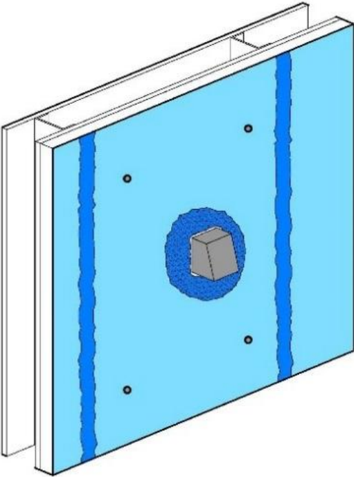
FIGURE 5—TYPICAL PENETRATION FLASHING DETAIL—FLANGED
