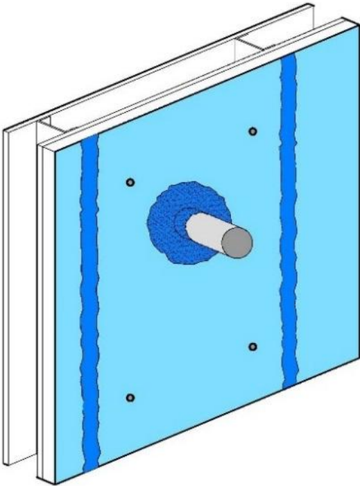
FIGURE 6—TYPICAL FLASHING DETAIL—UNFLANGED
