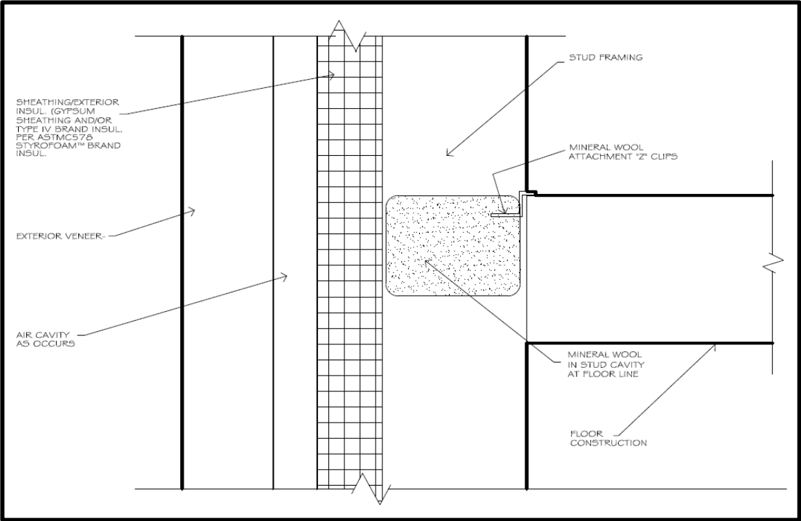
FIGURE 7—FLOORLINE FIRESTOPPING
