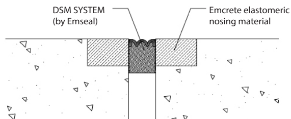
Figure 1: Emcrete Used as Expansion Joint Nosing Material
