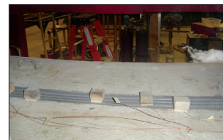
Thermocouples register no more than 248°F (120°C)
