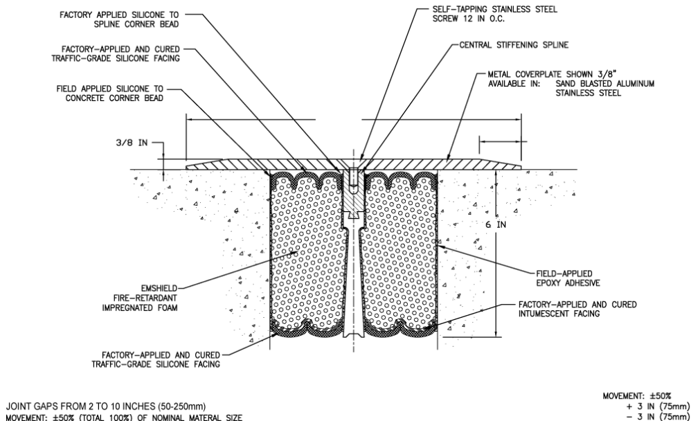
Figure 1: System Components (6-inch system for illustration. Available from 2-inch to 10-inch with Sealant Coating)
