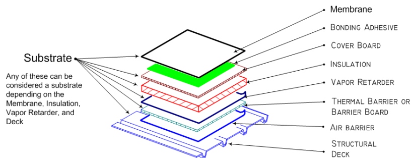
Diagram 1.01.1 Typical Roof Assembly Layers
