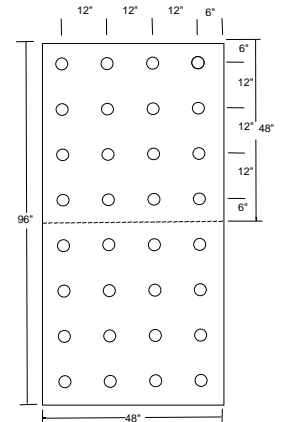
32 fasteners
