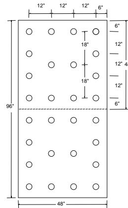
28 fasteners
