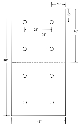
8 fasteners
