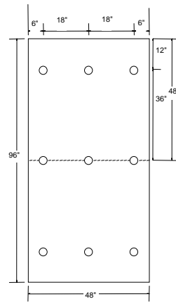
9 fasteners
