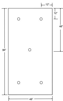
5 fasteners
