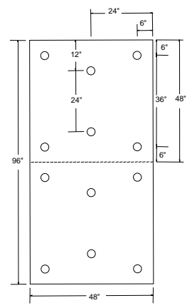
12 fasteners
