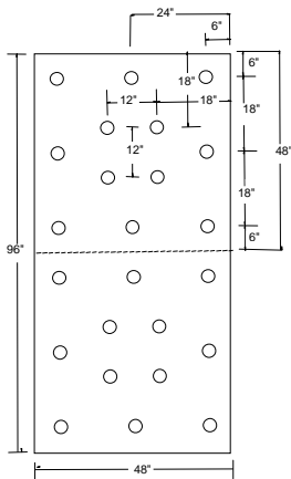
24 fasteners
