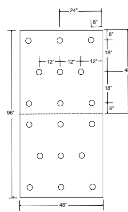
18 fasteners
