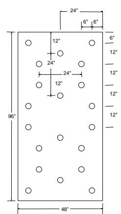
20 fasteners
