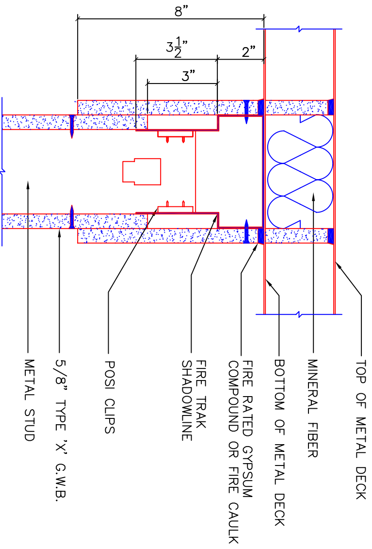
HEAD DETAIL - UL HW-D-1011 PERPENDICULAR TO METAL DECK 1 HR. RATING - 3" DEFLECTION
