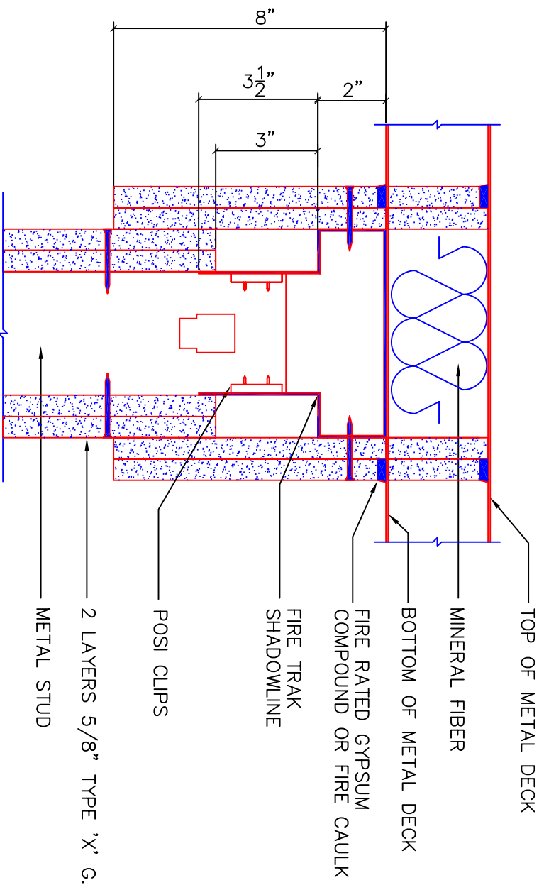
HEAD DETAIL - UL HW-D-1011 PERPENDICULAR TO METAL DECK 2 HR. RATING - 3" DEFLECTION
