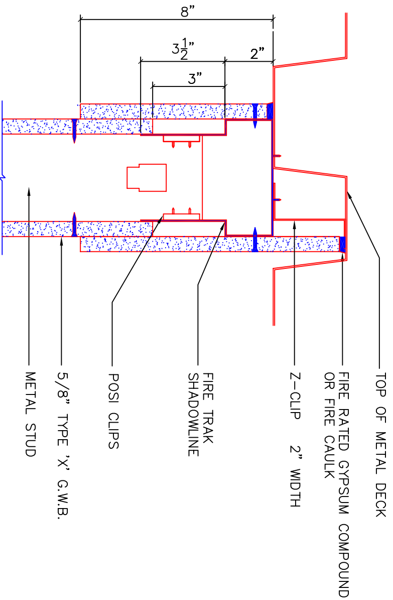
HEAD DETAIL – UL HW-D-1011 PARALLEL TO METAL DECK 1 HR. RATING – 3" DEFLECTION
