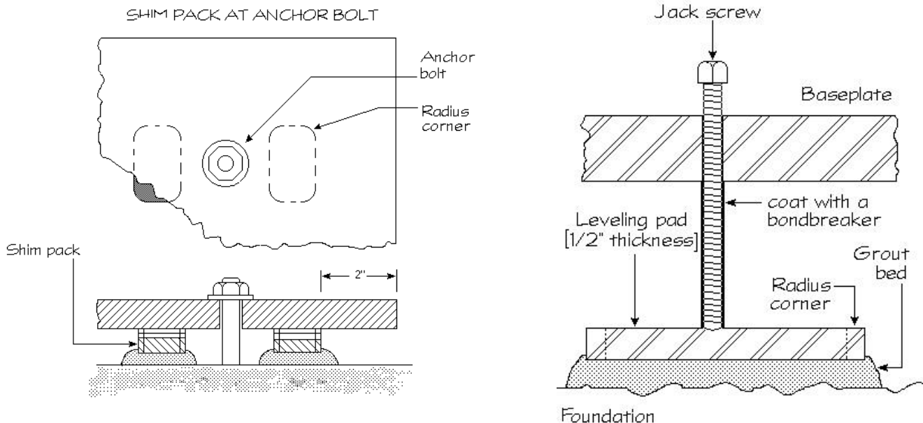
TYPICAL JACK SCREW DETAIL
