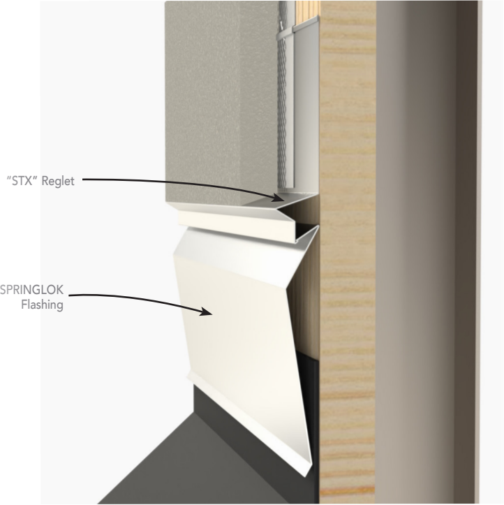
ASSEMBLY DETAIL
