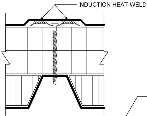
PLATE WELDED DETAIL
