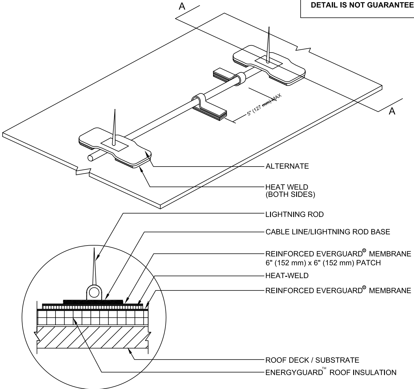
SECTION A
