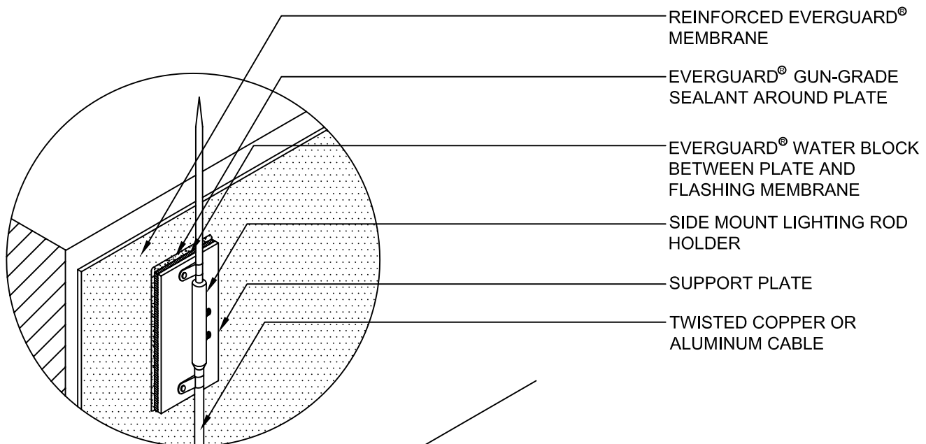
ALTERNATE ROD WALL MOUNT
