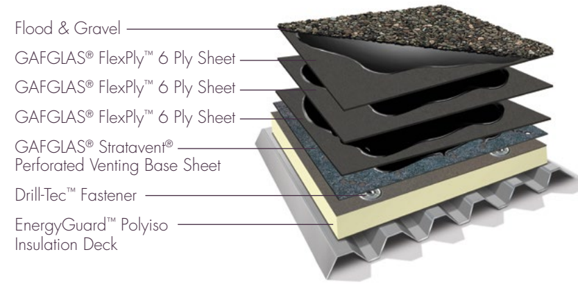
TYPICAL 4-PLY BUR SYSTEM WITH GAFGLAS® STRATAVENT®, FLEXPPLY™ 6, FLOOD COAT, AND GRAVEL
